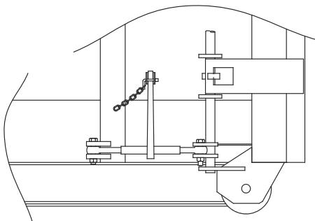
Ratchet locking gear
