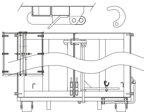
Multilift locking gear
