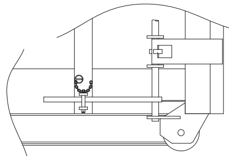
Lever locking gear
